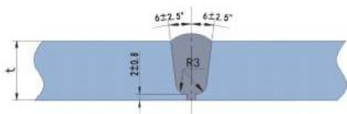
6 deg. U Type Beveling with 2mm Root, R= 5mm
